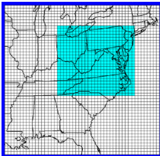
Figure 4: Early Action Modeling Domain of 36 km & 12 km Resolution
