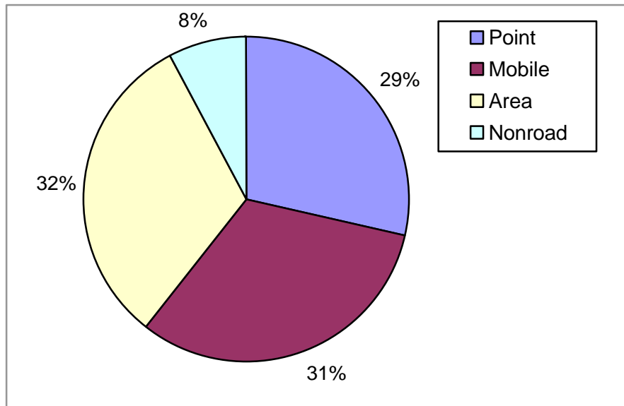
Figure 2: Northern Shenandoah Valley Emissions Inventory – 1999 Baseline Ozone Season Daily Emission of Volatile Organic Compounds (VOC)
